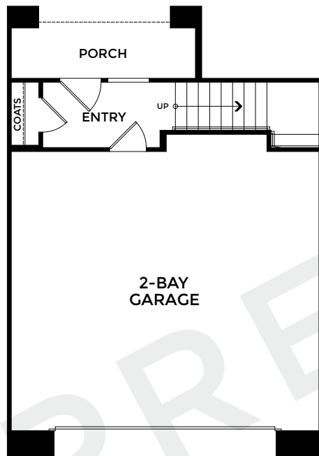
1ST FLOOR
