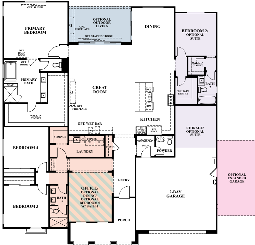
1ST FLOOR
