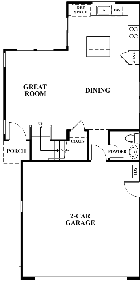
1ST FLOOR
