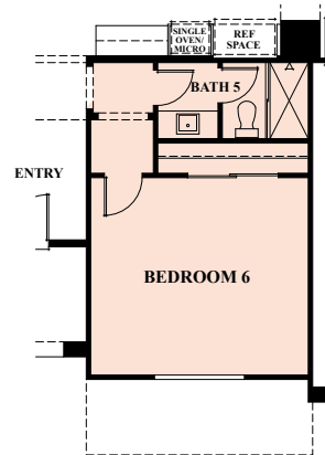
OPTIONAL BEDROOM 6 WITH BATH 5 IN LIEU OF OFFICE
