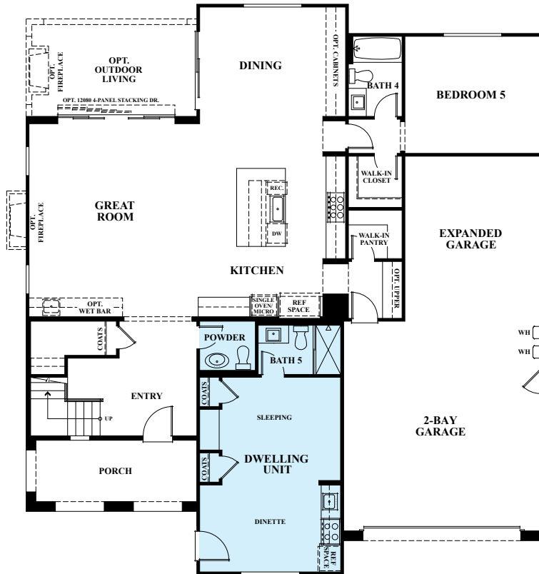
1ST FLOOR
